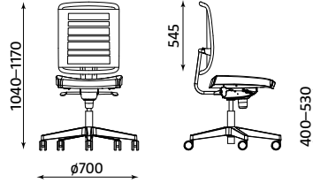
@-SENSE-PLUS-BL FS
