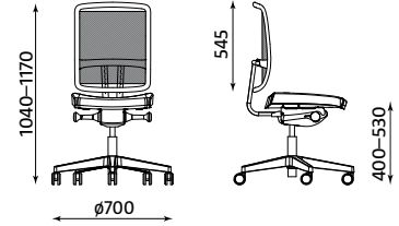
@-SENSE-BL LP11
