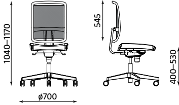
@-SENSE-BL FS
