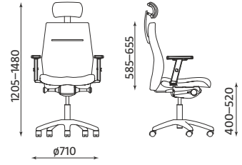
SO-ONE SWIVEL CHAIR UPH LB HRUA
