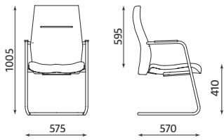
SO-ONE FRAME CHAIR CF UPH LB
